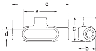
T shape
