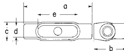
TB shape
