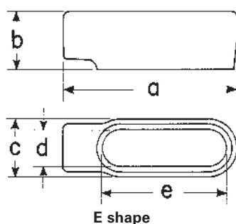
E shape
